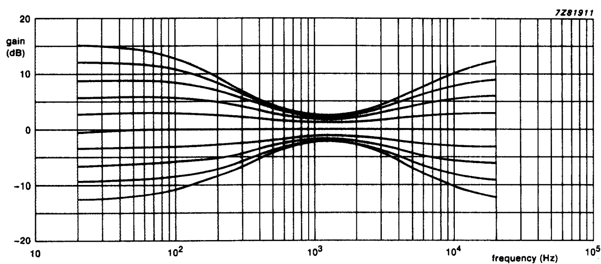
Fig.17 Frequency response of bass and treble control; bass and treble gain settings = -12 to +15 dB; gain is 0 dB; V_i = 0.1 V; R_{S9} = 600 \Omega ; R_L = 10 k \Omega ; V_{CC} = 12 V.
